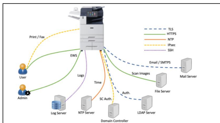
Figure 1: TOE Architecture
