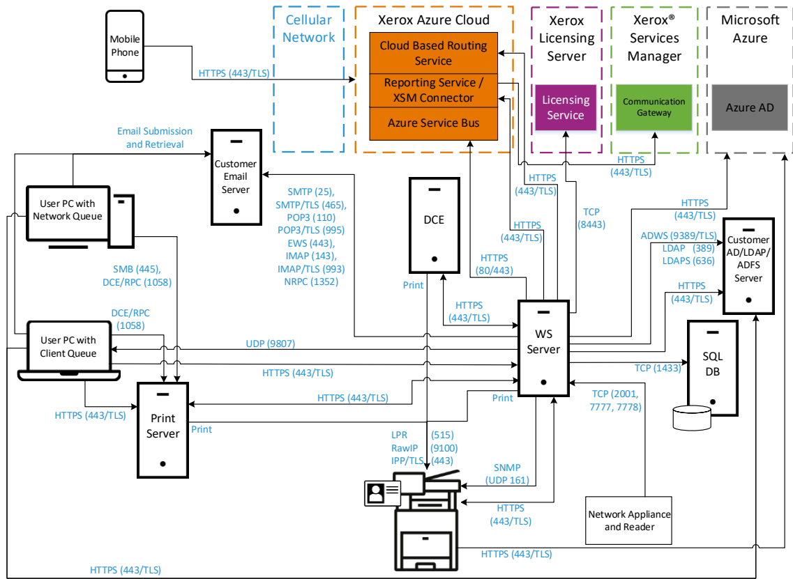
Xerox® Workplace Suite – Network Port Diagram
