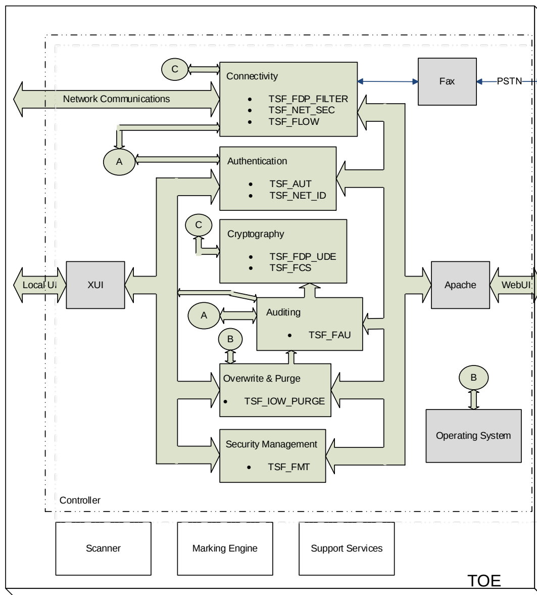
Figure 1 TOE Architecture
