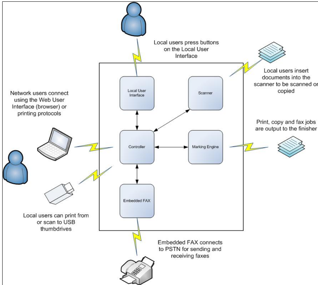
Figure 1: Architectural Diagram of the TOE
